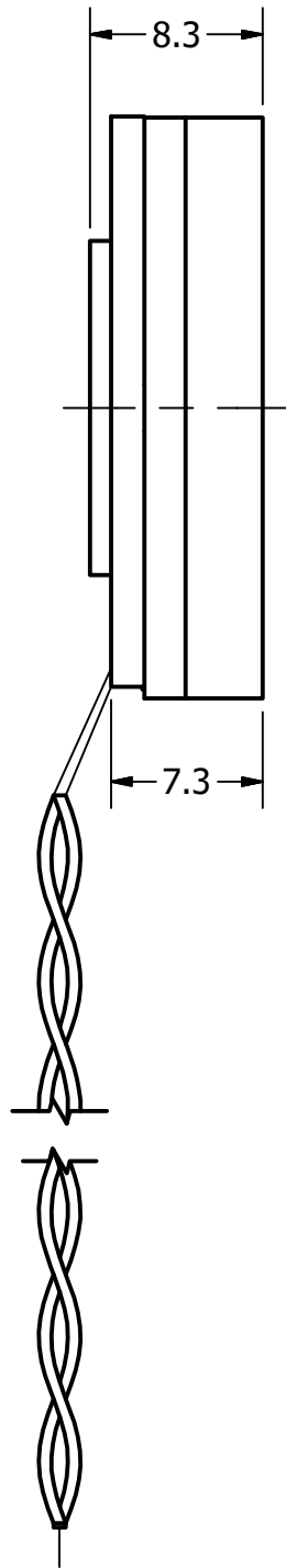
Side View
