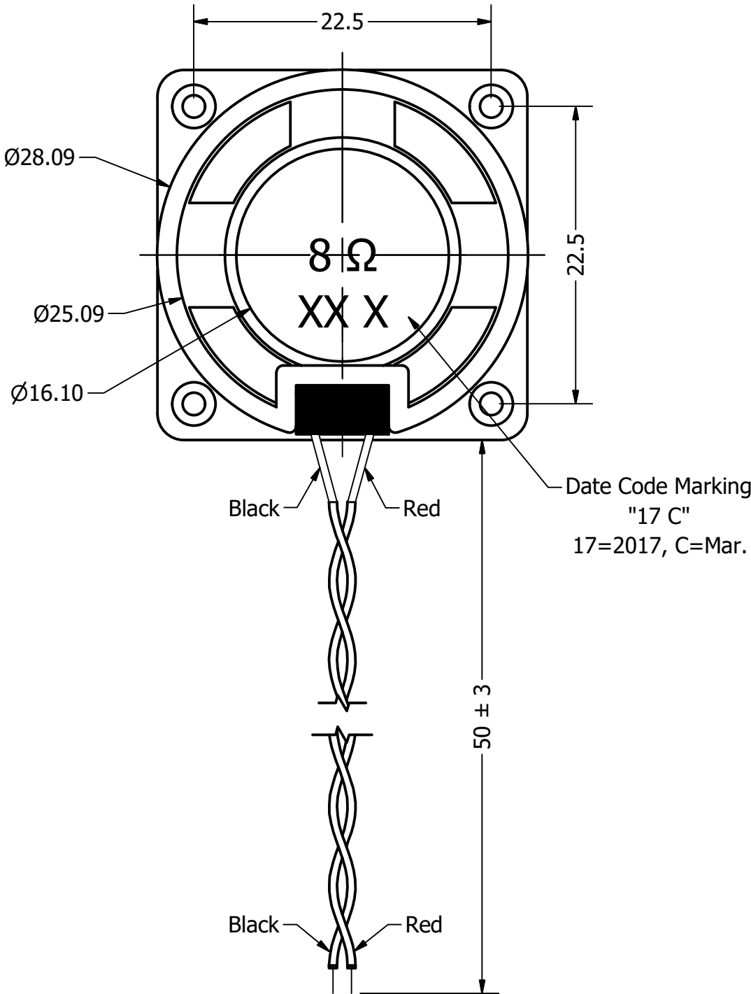
Bottom View
