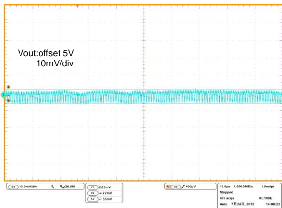
Figure 29. Lx Switching/ Vout Ripple
