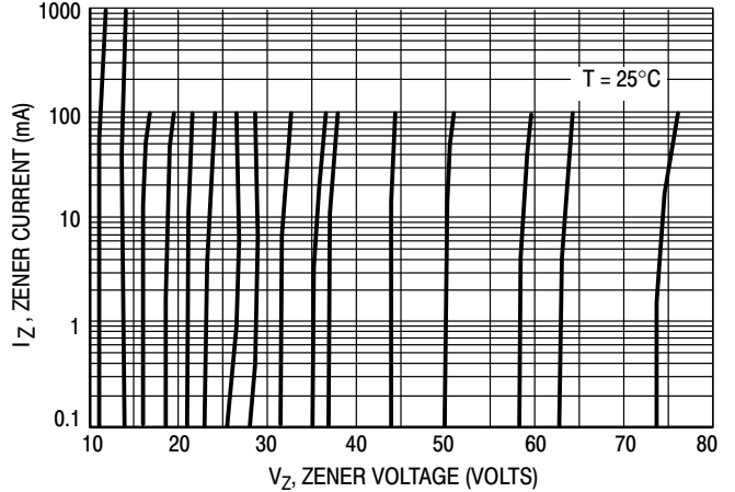
Figure 8. Zener Voltage versus Zener Current V_Z = 11 \text{ thru } 75 \text{ Volts}
