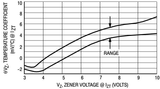
Figure 2. Temperature Coefficient-Range for Units 3 to 10 Volts
