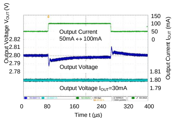
Load Transient Response Waveforms
