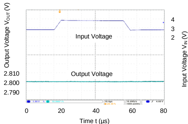
Line Transient Response Waveforms
