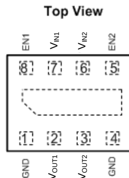
X2-DFN1612-8
