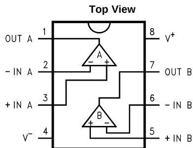
Figure 60. 8-Pin VSSOP/SOIC Package
