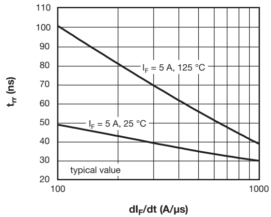
Fig. 6 - Typical Reverse Recovery vs. di/dt
