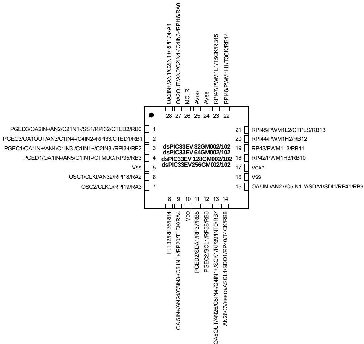
28-Pin QFN-S (1,2,3,4)
