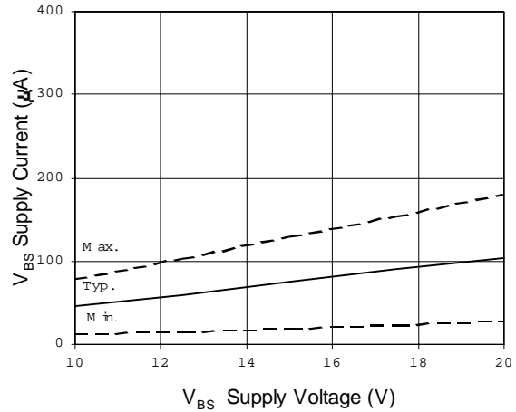
Figure 13B. V_{BS} Supply Current vs. Supply Voltage
