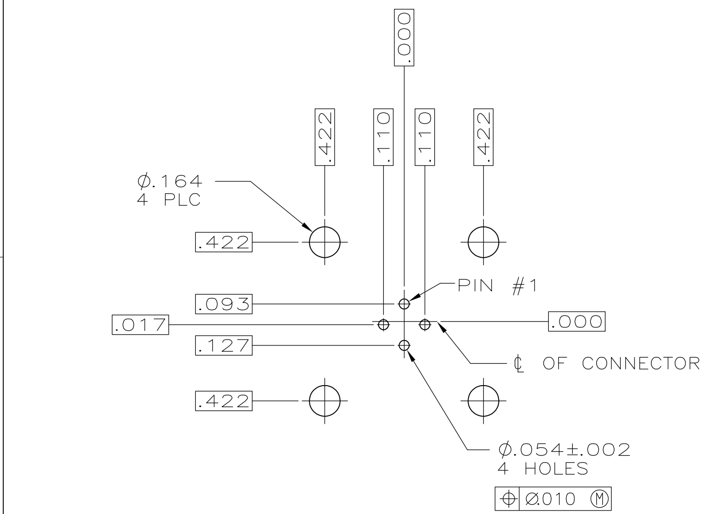
RECOMMENDED P.C. BOARD LAYOUT
