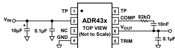
Figure 32. Compensated Reference
