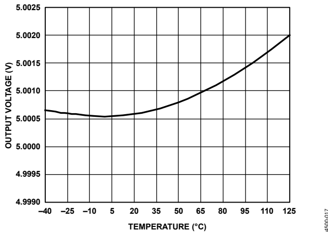
Figure 5. ADR435 Output Voltage vs. Temperature
