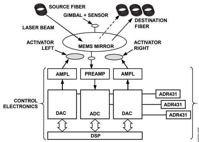
Figure 35. All Optical Router Network
