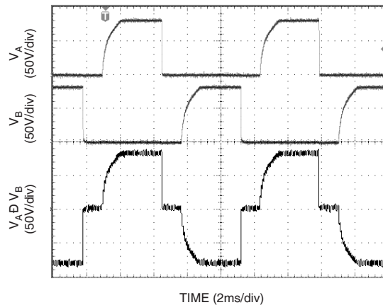
Figure 5. Typical 100Hz EL Driver for 3\text{in}^2 Lamp
