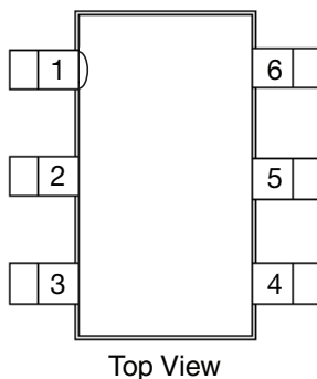
Figure 3 - TSOT23-6 Package
