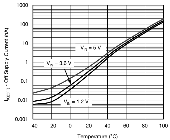
Figure 9 - Off Supply Current vs. Temperature
