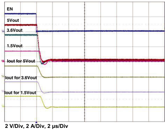
Figure 23 - Typical Fall Time C_{OUT} = 0.1 \mu F , C_{IN} = 4.7 \mu F , I_{OUT} = 1.5 A
