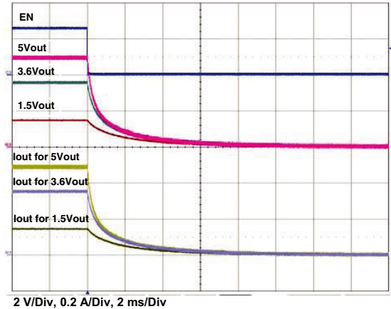
Figure 29 - Typical Fall Time C_{OUT} = 200 \mu\text{F} , C_{IN} = 4.7 \mu\text{F} , R_{OUT} = 10 \Omega
