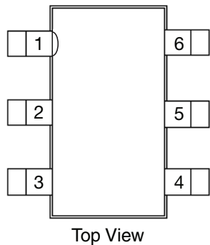
Figure 3 - TSOT23-6 Package
