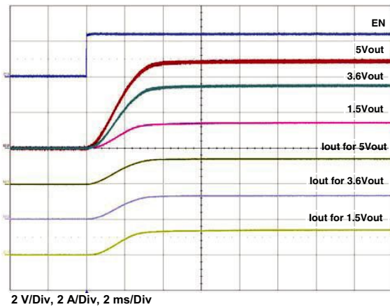
Figure 27 - Typical Turn-on Delay, Rise Time C_{OUT} = 100 \mu\text{F} , C_{IN} = 4.7 \mu\text{F} , I_{OUT} = 1.5 \text{ A}
