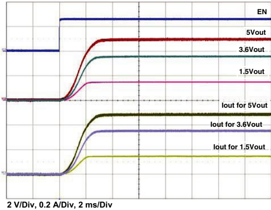
Figure 26 - Typical Turn-on Delay, Rise Time C_{OUT} = 200 \mu\text{F} , C_{IN} = 4.7 \mu\text{F} , R_{OUT} = 10 \Omega
