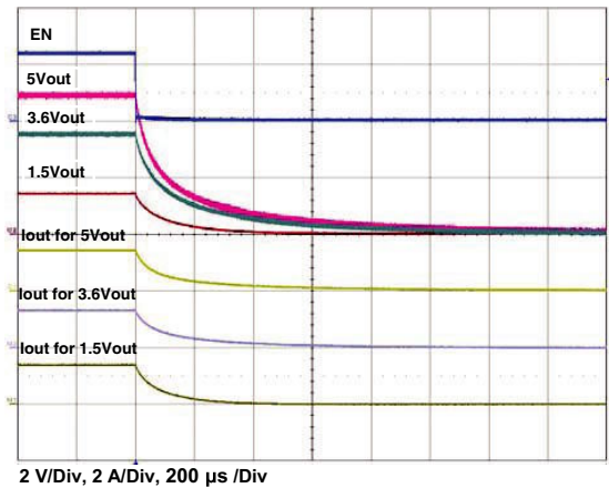
Figure 30 - Typical Fall Time C_{OUT} = 100 \mu\text{F} , C_{IN} = 4.7 \mu\text{F} , I_{OUT} = 1.5 \text{ A}
