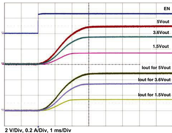
Figure 28 - Typical Turn-on Delay, Rise Time C_{OUT} = 100 \mu\text{F} , C_{IN} = 4.7 \mu\text{F} , R_{OUT} = 10 \Omega
