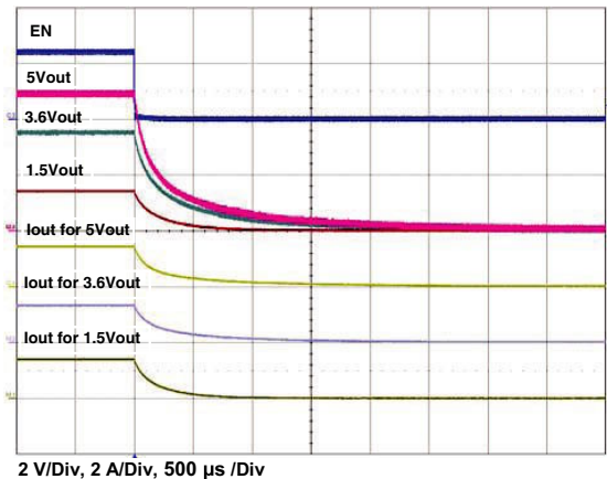
Figure 25 - Typical Fall Time C_{OUT} = 200 \mu F , C_{IN} = 4.7 \mu F , I_{OUT} = 1.5 A
