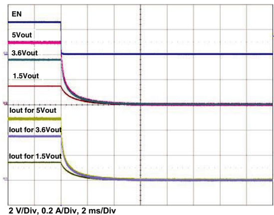
Figure 31 - Typical Turn-on Delay, Fall Time C_{OUT} = 100 \mu\text{F} , C_{IN} = 4.7 \mu\text{F} , R_{OUT} = 10 \Omega
