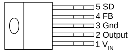
TO220-5L/TO220-5L(R)
