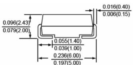
SMA/DO-214AA
