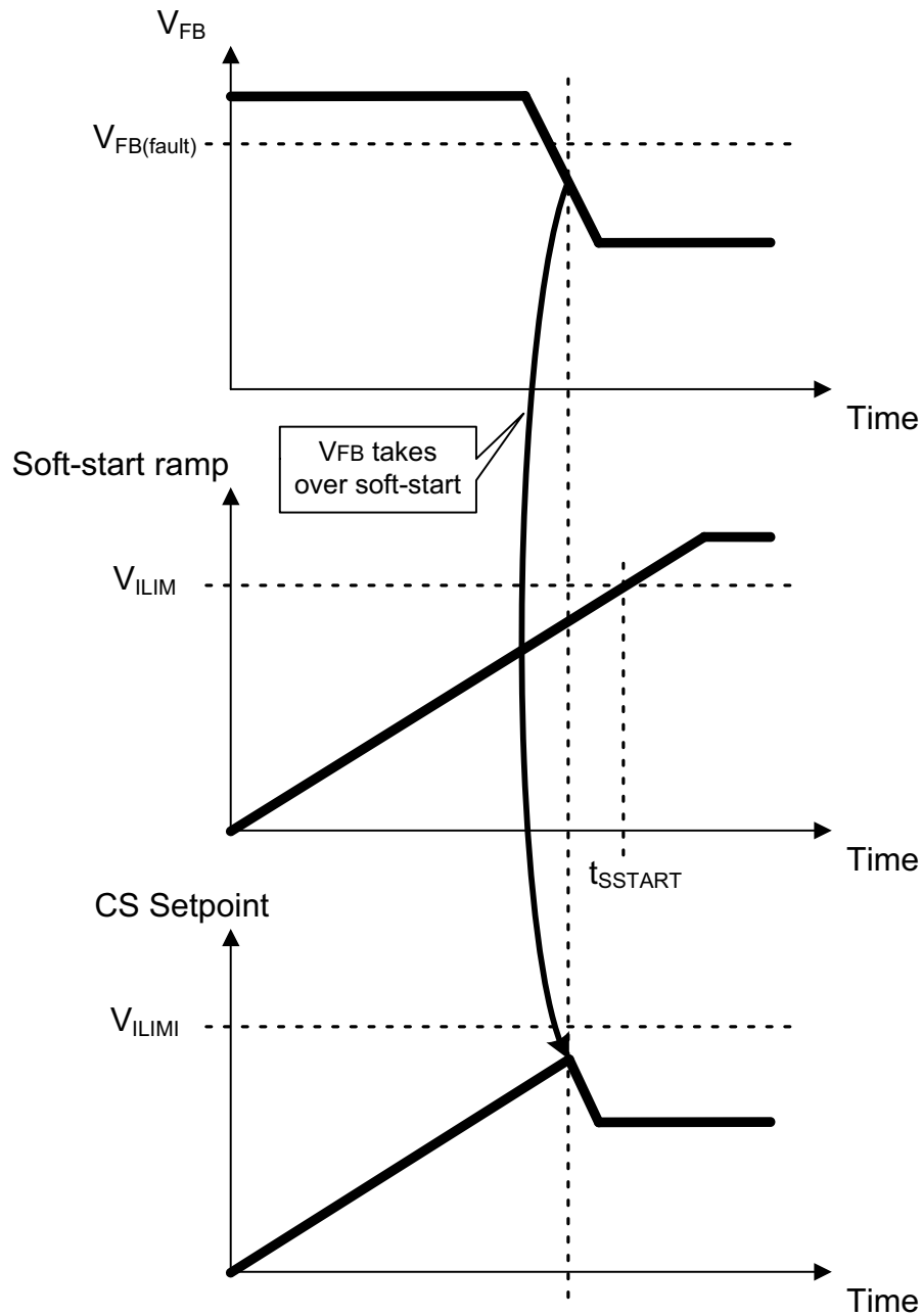
Figure 37. Soft-Start
