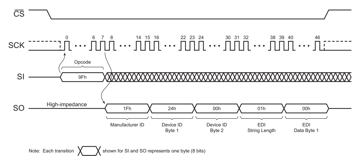
Figure 12-1. Read Manufacturer and Device ID
