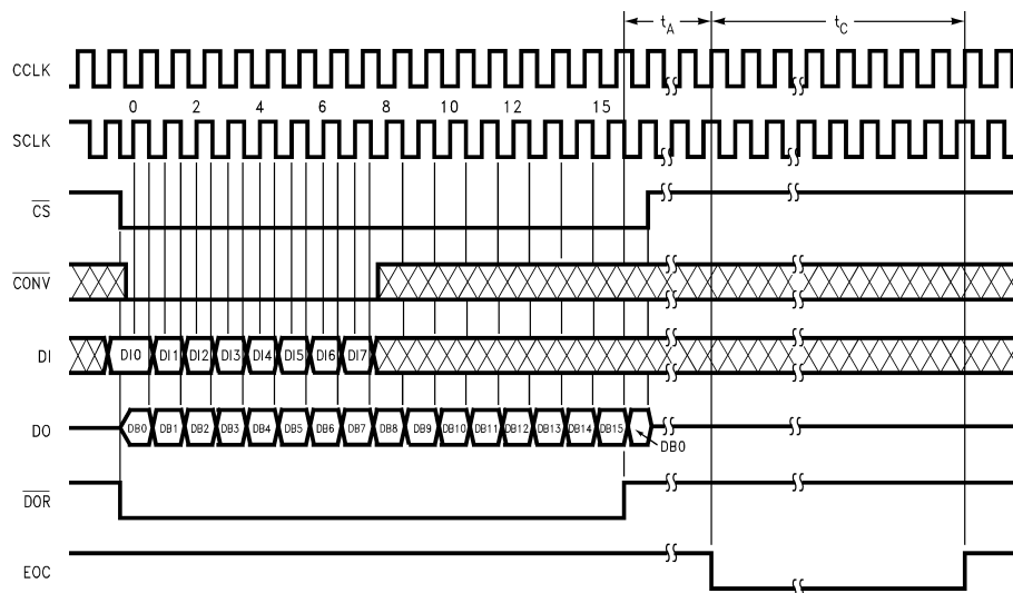
Figure 29. ADC12L038 Conversion Using \overline{\text{CS}} with 16-Bit Digital Output Format
