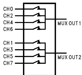
Differential Configuration
