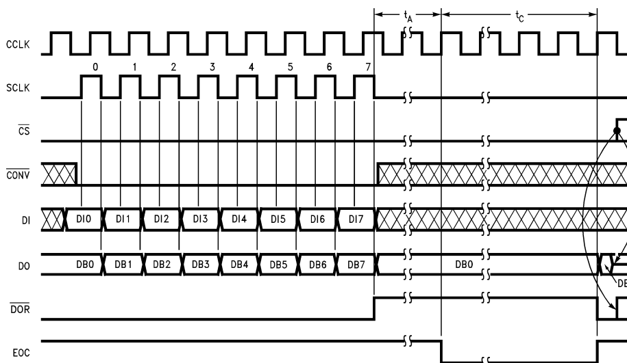
Figure 30. ADC12L038 Conversion with \overline{\text{CS}} Continuously Low and 8-Bit Digital Output Format
