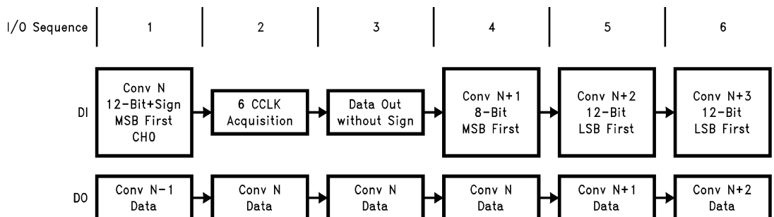
Figure 39. Changing the ADC's Conversion Configuration
