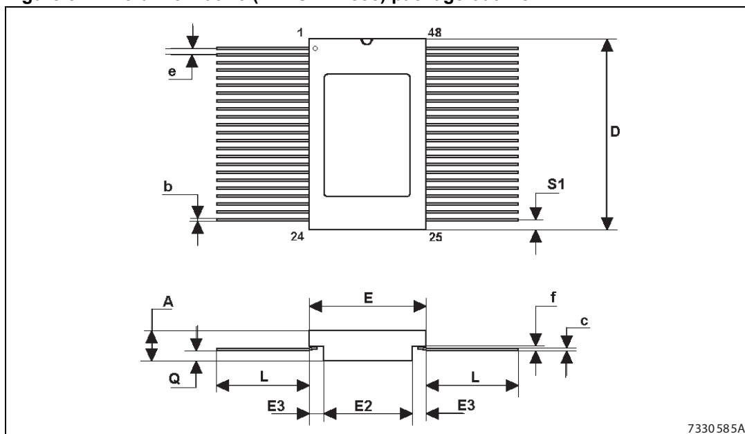
Figure 8. Ceramic Flat-48 (MIL-STD-1835) package outline
