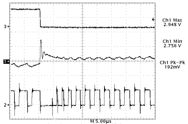
Figure 11. CS5157H Demonstration Board Response to 13 A Load Turn Off (Output Set for 2.8 V). V^2 Control Topology Immediately Connects Inductor to Ground, Providing 0% Duty Cycle. Regulation is Achieved in Less Than 10 \mu s
