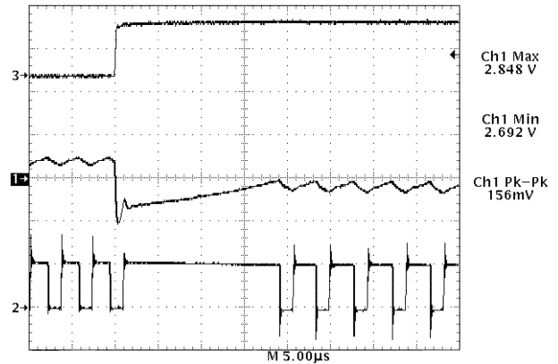
Figure 10. CS5157H Demonstration Board Response to 13 A Load Turn On (Output Set for 2.8 V). Upon Completing a Normal Off Time, The V^2 Control Loop Immediately Connects the Inductor to the Input Voltage, Providing 100% Duty Cycle. Regulation is Achieved in Less Than 20 \mu s
