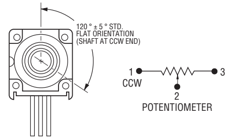
Shaft Flat Orientation
