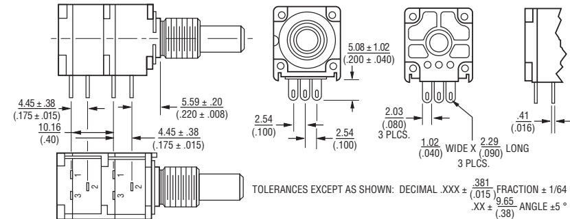
Model 95 Solder Lug Terminals, "Triangular" Pattern
