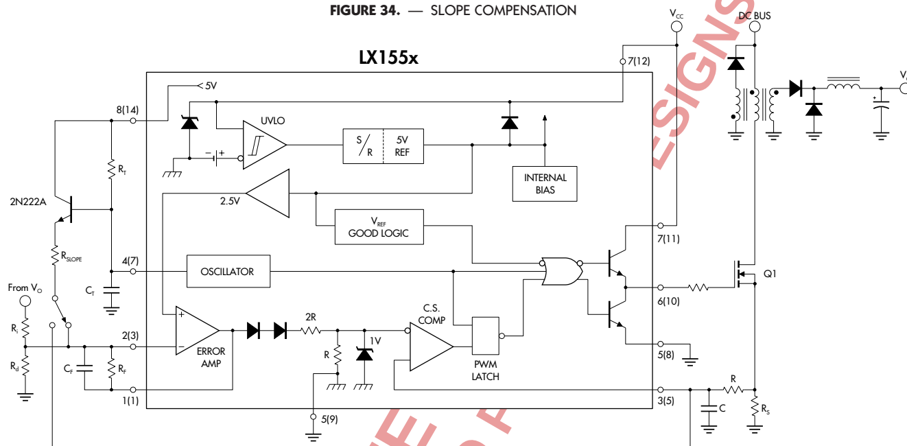
FIGURE 34. — SLOPE COMPENSATION
