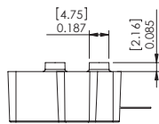
B- Two Ports Cut 0.085" Configuration
