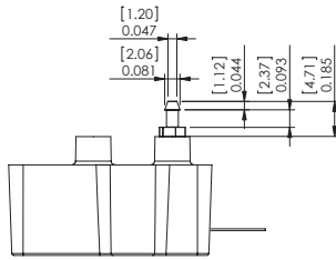
B- Barb Fitting Port A Only Configuration
