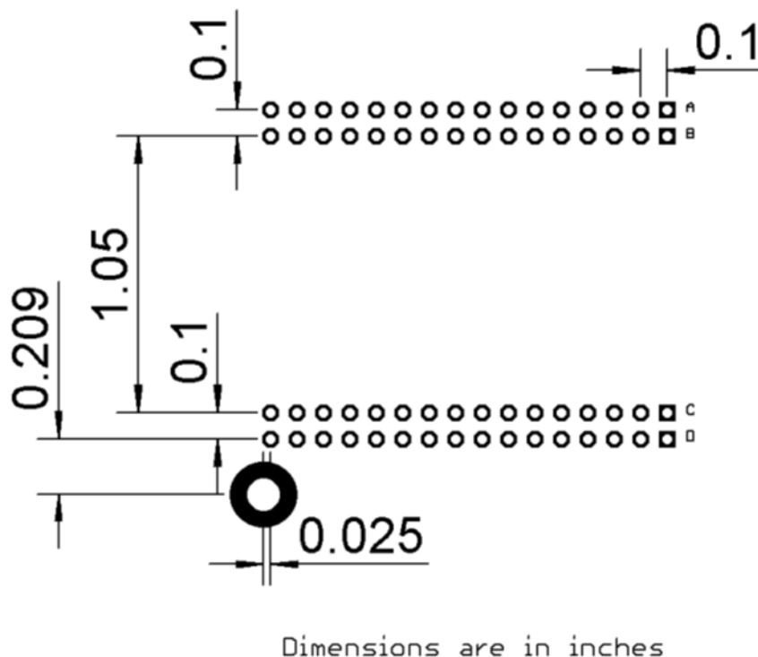
Figure 4 - Socket dimensions to mate the DLR Network Interface Module
