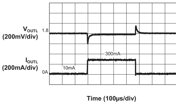
LDO Load Transient (VIN = 3.6V; VOUTL = 1.8V; CINL = 2.2μF; COUTL = 1μF)
