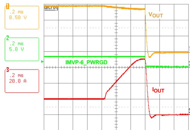
FIGURE 23. OVERCURRENT PROTECTION
