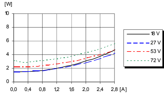
Dissipated power vs. load current and input voltage at T_{P1} = +25^{\circ}\text{C}
