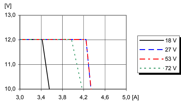
Output voltage vs. load current at I_O > \max I_O , T_{P1} = +25^{\circ}\text{C} The module enters hiccup mode when the output current exceeds current limit.
