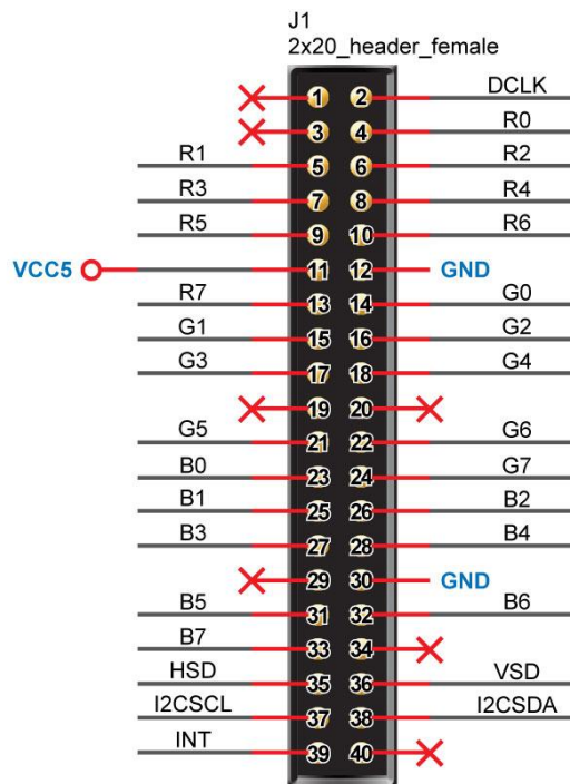
Figure 3-1 2x20 GPIO
