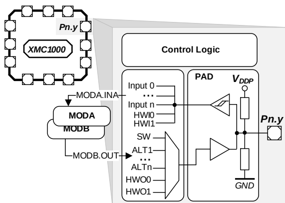
Figure 8 Simplified Port Structure
