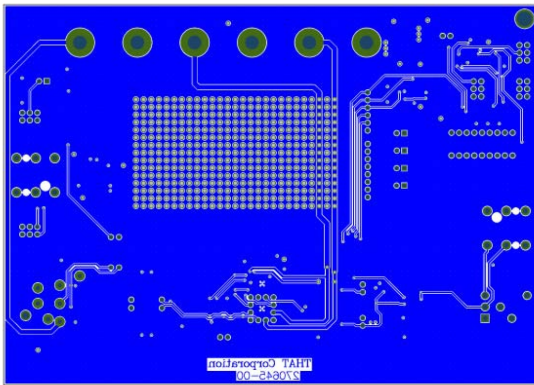
Layer 4 (Bottom)
