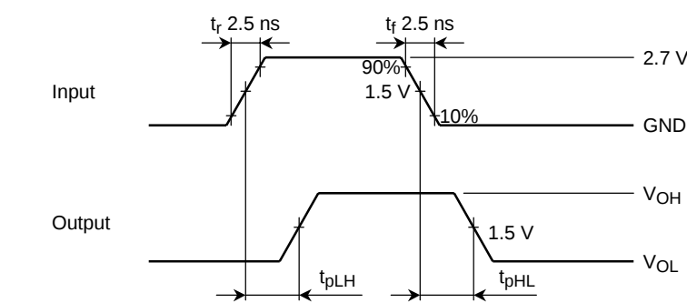
Figure 2 t_{pLH} , t_{pHL}
