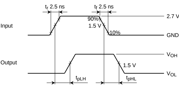
Figure 2 t_{pLH} , t_{pHL}
