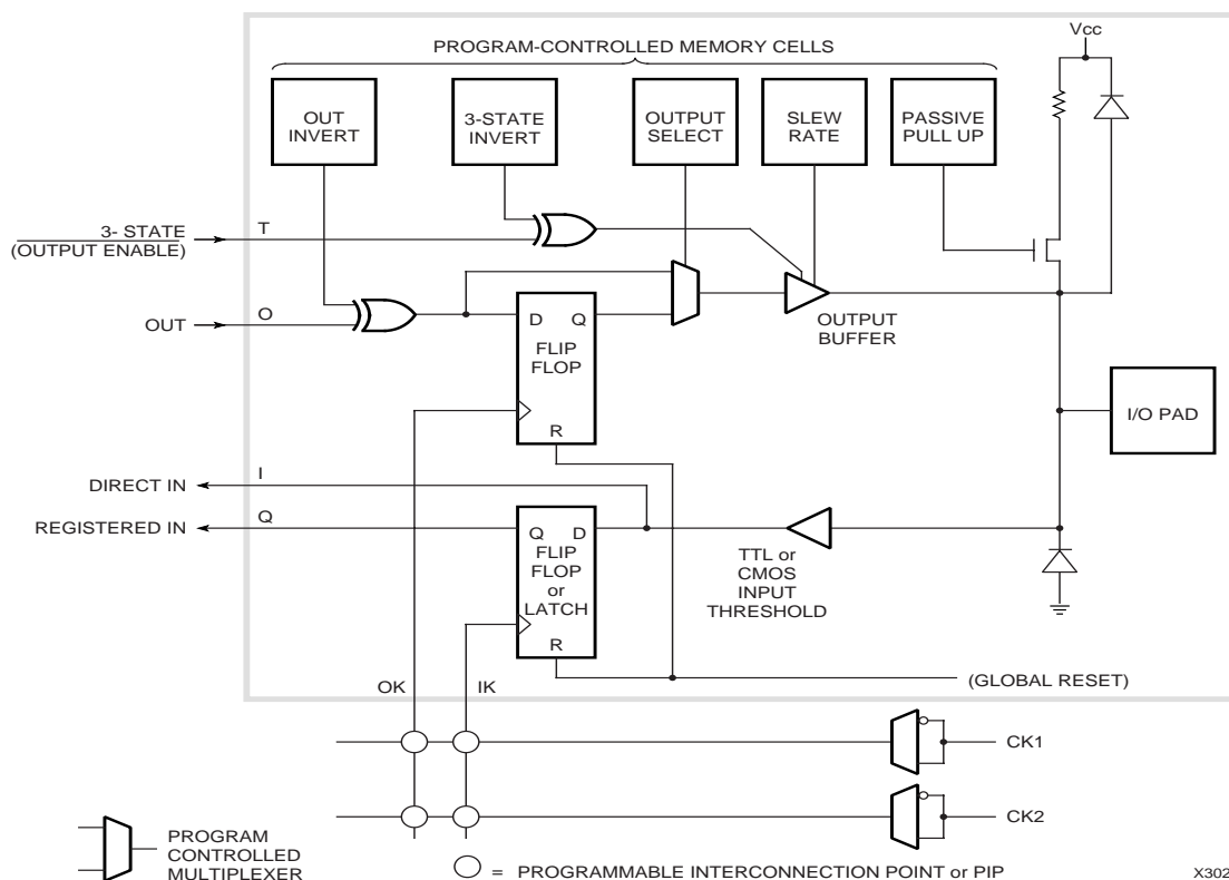
Each IOB includes input and output storage elements and I/O options selected by configuration memory cells. A choice of two clocks is available on each die edge. The polarity of each clock line (not each flip-flop or latch) is programmable. A clock line that triggers the flip-flop on the rising edge is an active Low Latch Enable (Latch transparent) signal and vice versa. Passive pull-up can only be enabled on inputs, not on outputs. All user inputs are programmed for TTL or CMOS thresholds.
