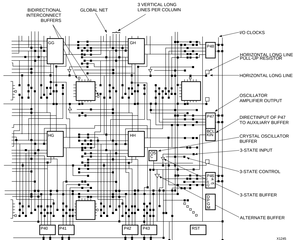
Figure 18: Design Editor.
