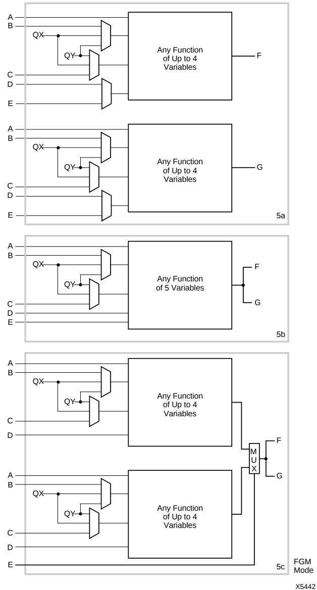
Figure 6: Combinational Logic Options
