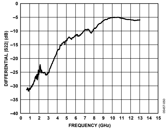
Figure 10. Differential |S22|
