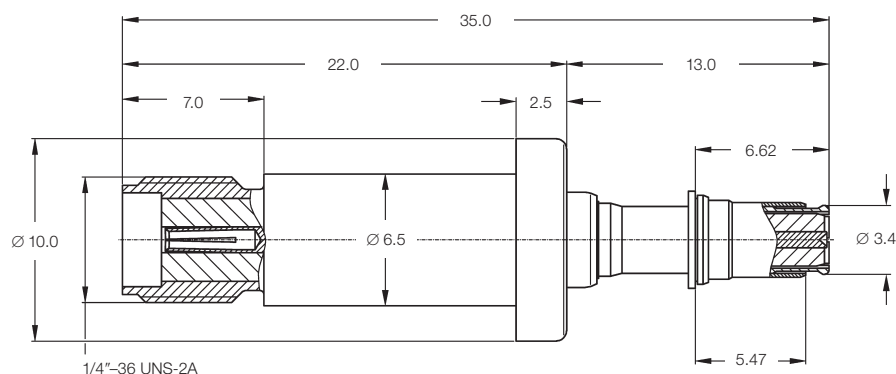
Part No. 619052-1
