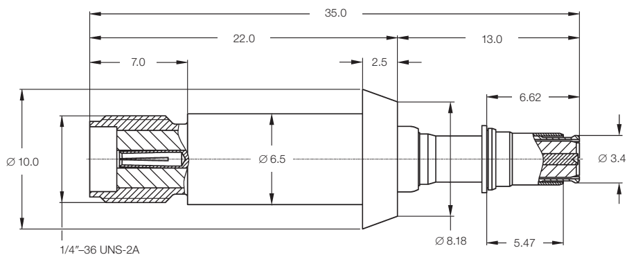
Part No. 619052-1
