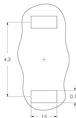
PCB Layout
