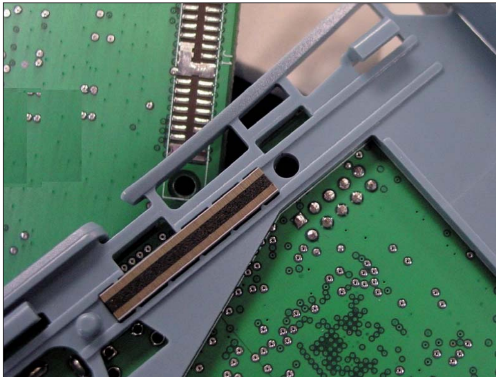
Dual-Row STAX Connector connects two rows of contact pads. Retention slot is provided in PCB separator.
