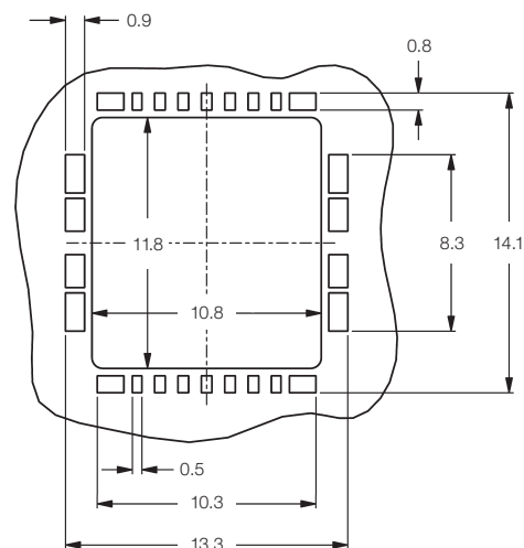
PCB Layout
