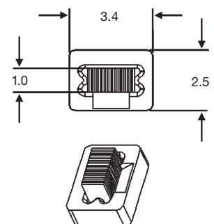
Part No. 1-1442004-7
