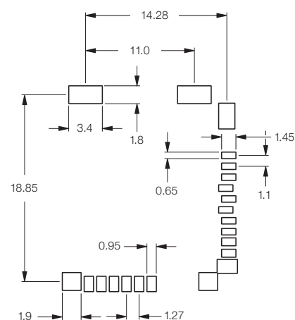
PCB Layout
