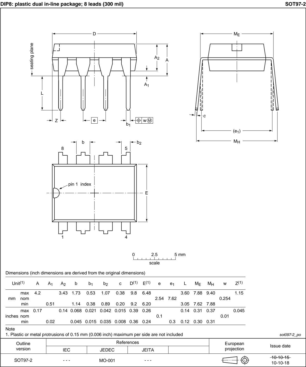
Fig 36. Package outline SOT097-2 (DIP8)
