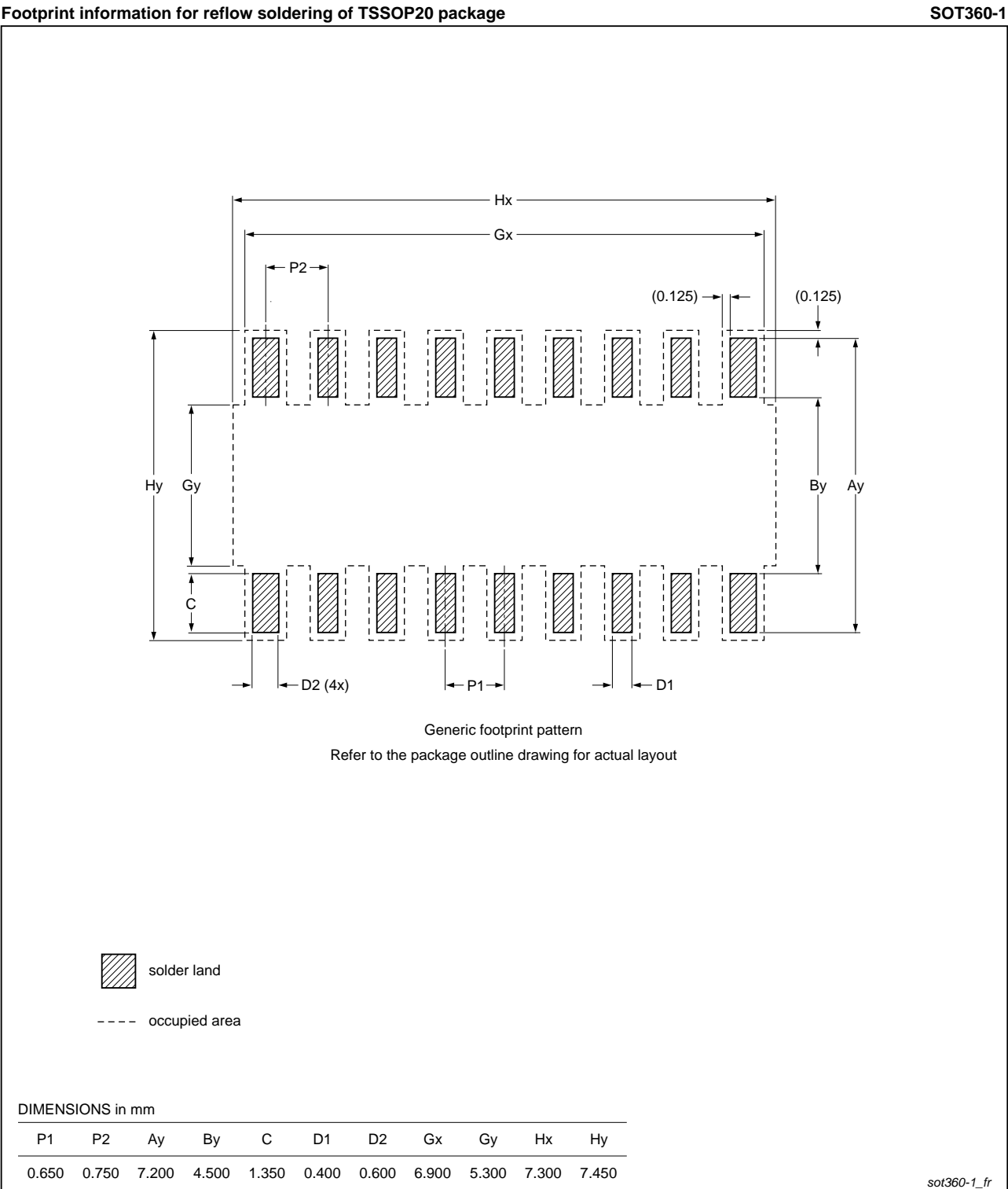
Fig 42. Reflow soldering of the TSSOP20 package
