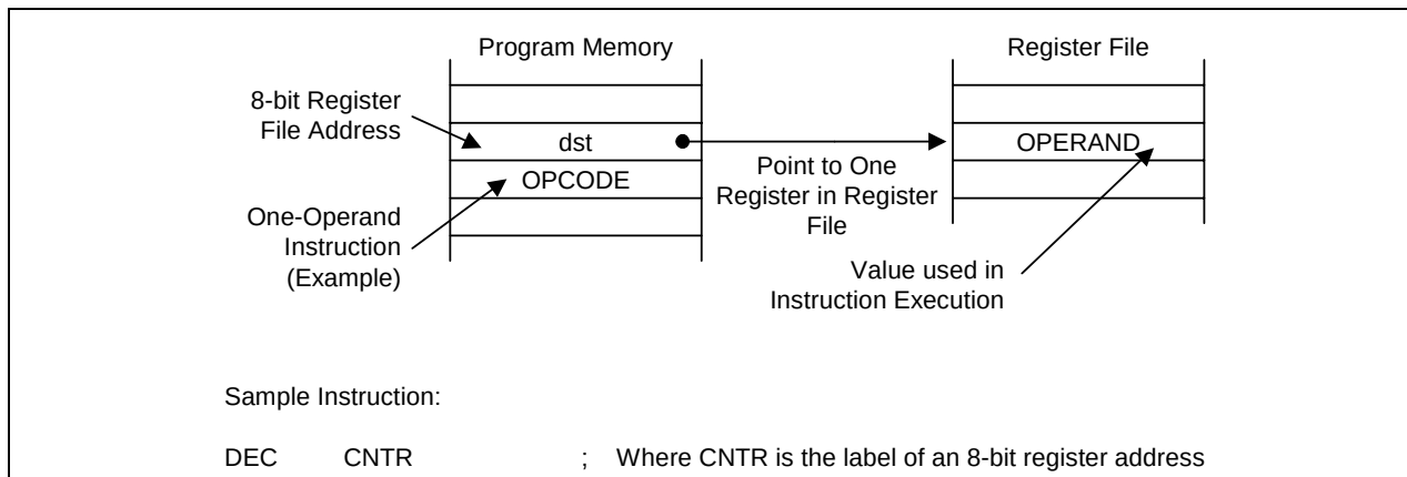
Figure 3-1. Register Addressing
