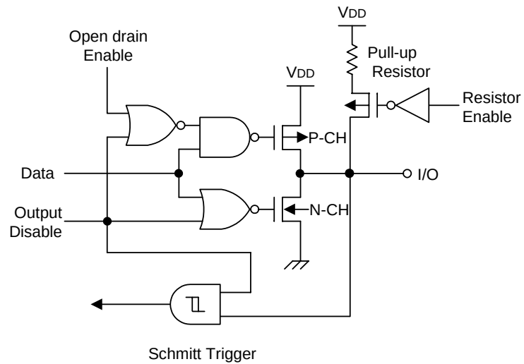
Figure 1-8. Pin Circuit Type E-4 (P1.0-P1.3)
