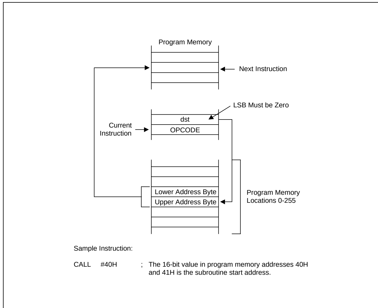
Figure 3-12. Indirect Addressing
