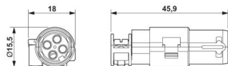
Female insert
