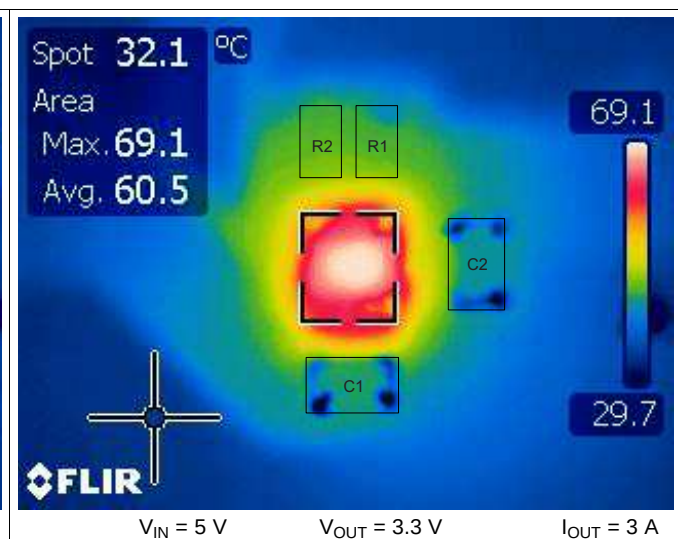
Figure 25. Thermal Measurement
