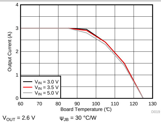
Figure 10. Thermal Derating
