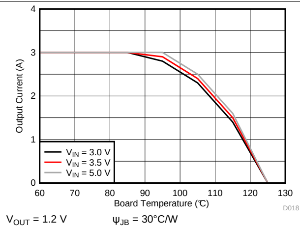
Figure 9. Thermal Derating
