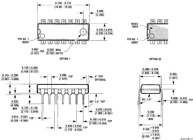
14-Lead Plastic Dual-In-Line Package (N) NS Package Number N14A
