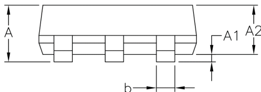
BOTTOM VIEW
