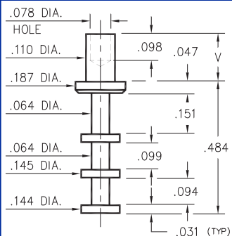
2806-X-00-XX-00-00-07-0 Swage mount in .116 hole
