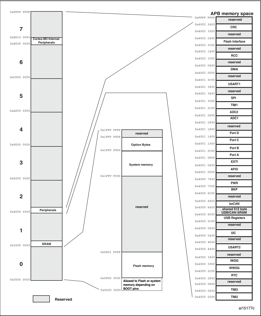
Figure 8. Memory map
