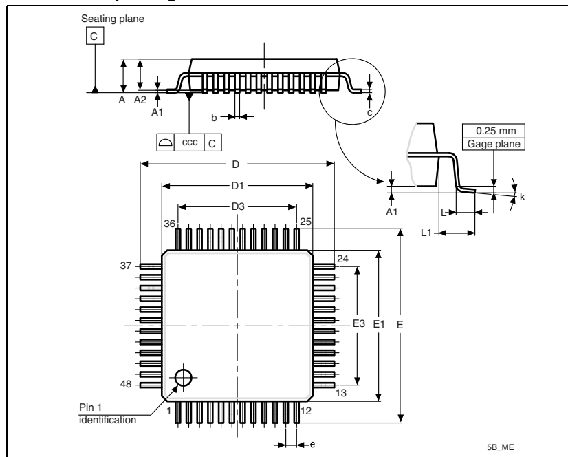
Figure 46. LQFP48, 7 x 7 mm, 48-pin low-profile quad flat package outline (1)
