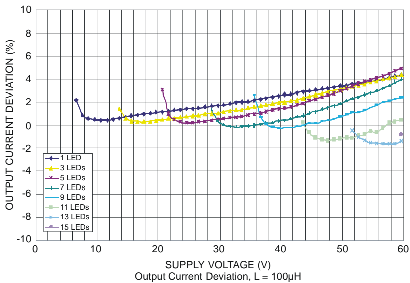
Output Current, L = 100μH
