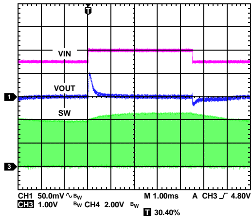
Figure 23. BUCK1 Response to Line Transient, Input Voltage from 4.5 V to 5.0 V, V_{OUT1} = 3.3\text{ V} , PWM Mode
