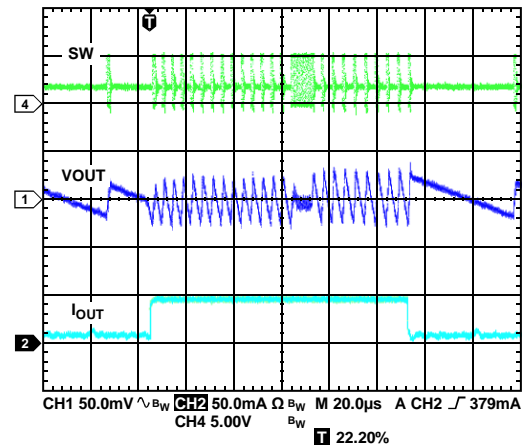
Figure 26. BUCK2 Response to Load Transient, I_{OUT2} from 1 mA to 50 mA, V_{OUT2} = 1.8\text{ V} , Automatic Mode
