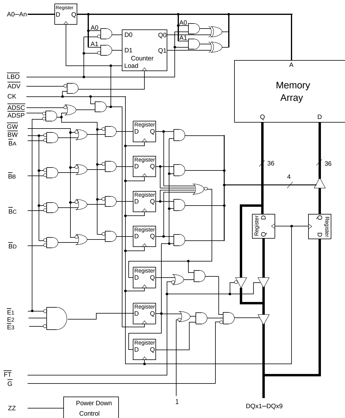
GS8320E18/32/36AGT Block Diagram
