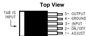
Figure 2. DDPak, TO-263 Package, 5-Lead, Surface-Mount See Package Number KTT
