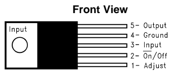
Figure 1. TO-220 Package, 5-Lead See Package Number KC and NDH
